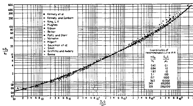
Fig. 3. Original correlation for convection between a gas stream and a cylinder (5).
